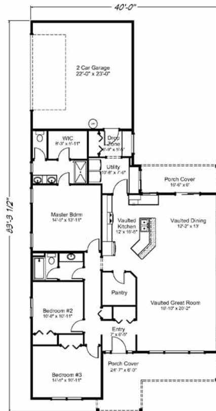
Whispering Fires 1829 sq. ft. • 3 bedrooms • 2 baths • 2 car garage
